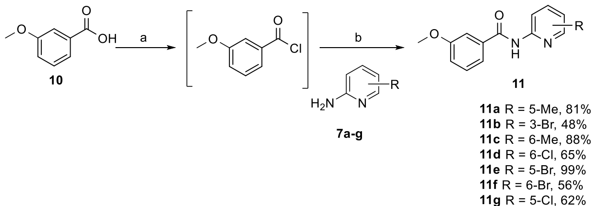
Scheme 3. Reagents and conditions: a) \text{SOCl}_2 , reflux, 24 h; b) aminopyridine, pyridine, 0 °C – rt, 10 – 24 h, 48 – 99%.
