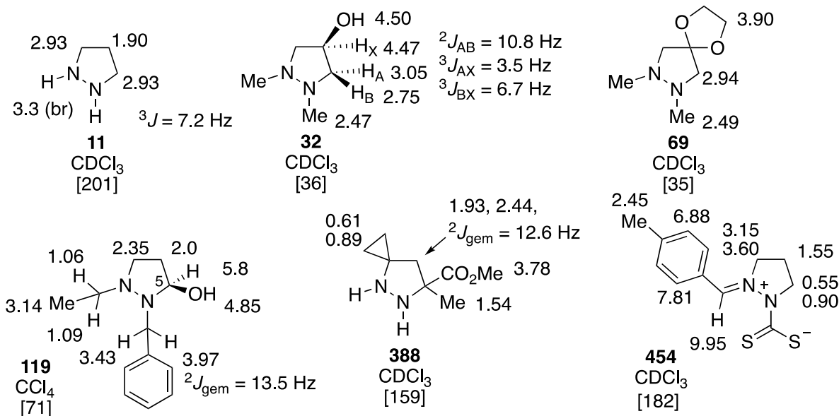
Figure 13. ^1\text{H} chemical shifts of some interesting molecules.
