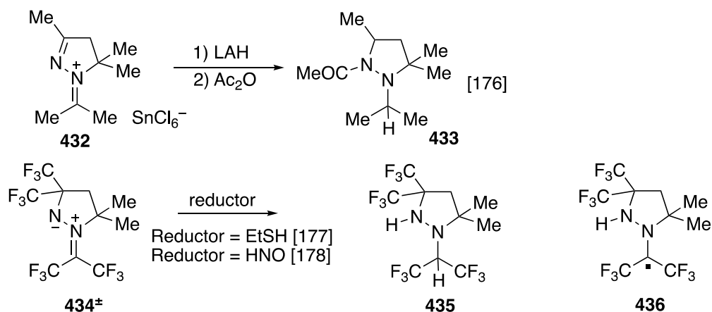
Scheme 23. Reduction of compound 432 , related to cation 385 , and zwitterion 434 ± .
