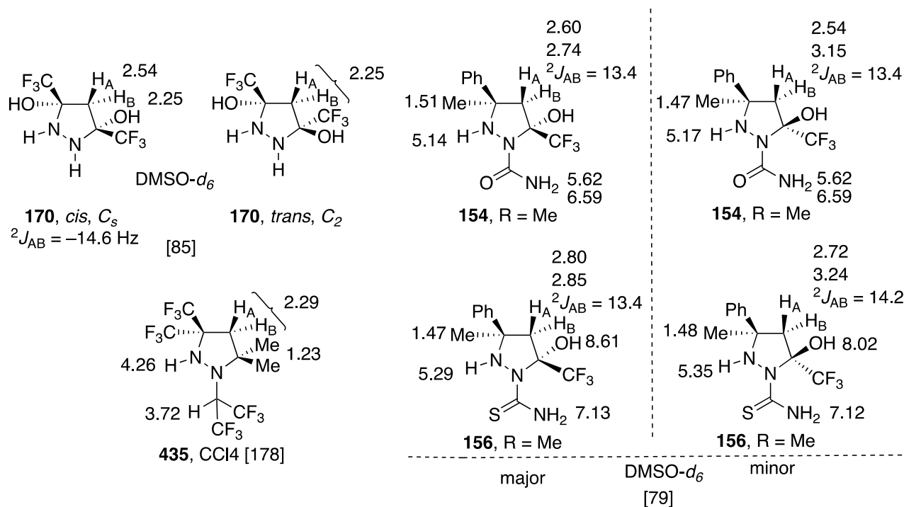
Figure 12. Some ^1\text{H} NMR data of fluorinated pyrazolidines.
