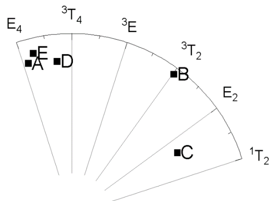
Figure 20. The five more stable conformation of 31 .
