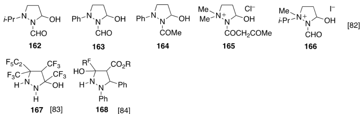
Figure 4. Other 5-hydroxypyrazolidines.
