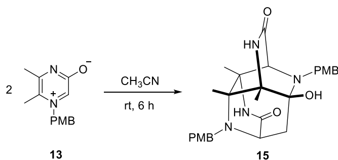
Scheme 5. Dimerization of 3-oxidopyrazinium 13 .
