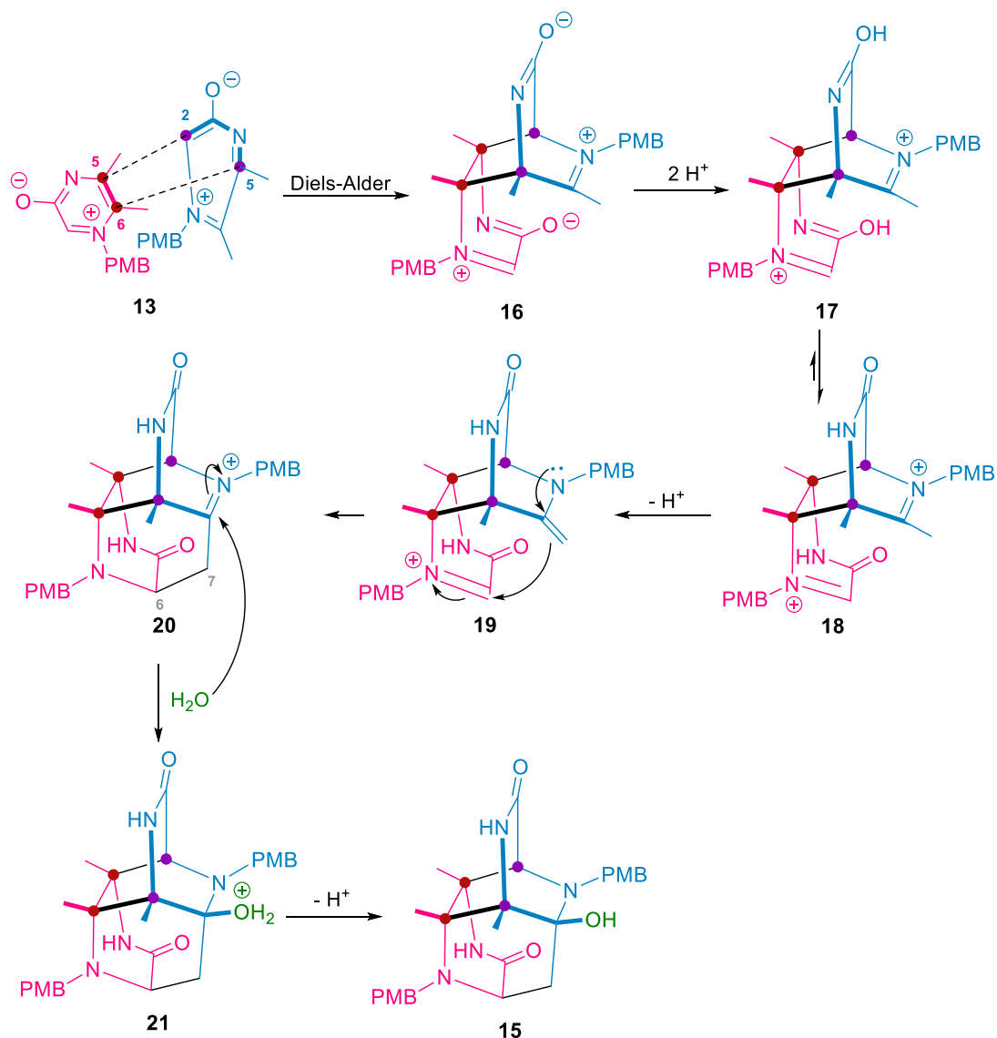
Scheme 6. Proposed mechanism of formation of the dimer 15 from 13 .
