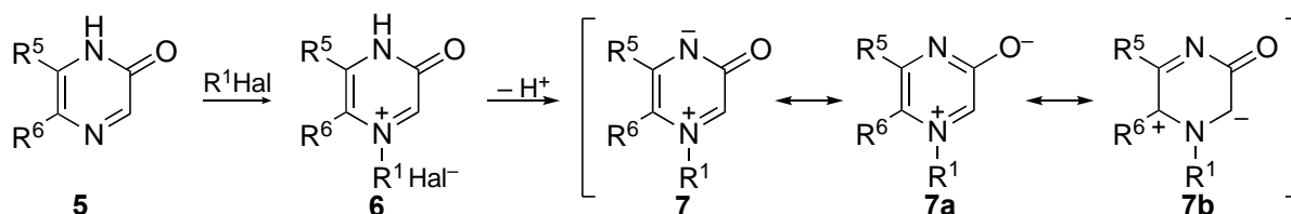
Scheme 2. Main resonance contributors to 3-oxidopyraziniums 7 and synthesis from 2(1 H )-pyrazinones 5 .
