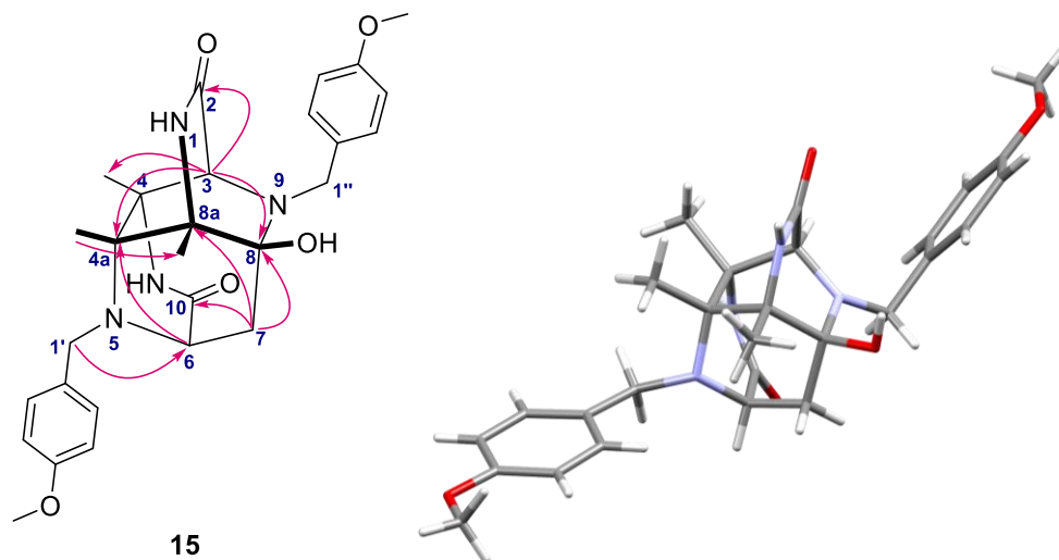
Figure 1. Selected key 1 H- 13 C HMBC correlations and capped-stick representation of the X-ray crystal structure of 15 .
