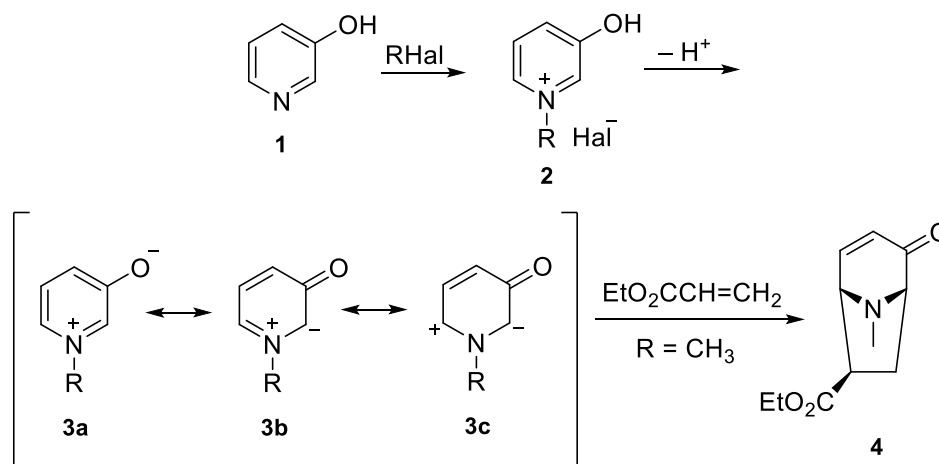
Scheme 1. Main resonance contributors to 3-oxidopyridiniums and reaction of 1-methyl-3-oxidopyridinium 3 ( R = \text{Me} ) with ethyl acrylate.
