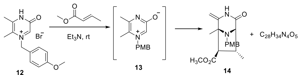
Scheme 4. Cycloaddition between 3-oxidopyrazinium 13 and methyl crotonate.
