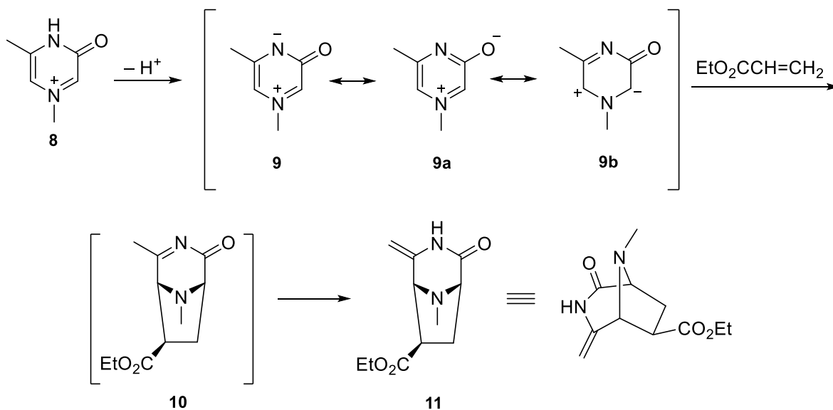
Scheme 3. Synthesis of 1,5-dimethyl-3-oxidopyrazinium ( 9 ) and its reaction with ethyl acrylate.
