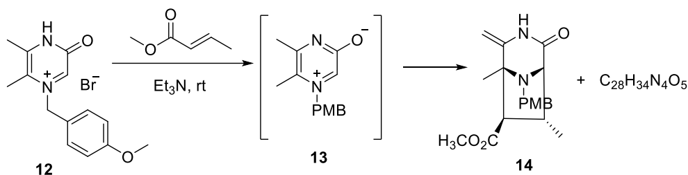
Scheme 4. Cycloaddition between 3-oxopyrazinium 13 and methyl crotonate.
