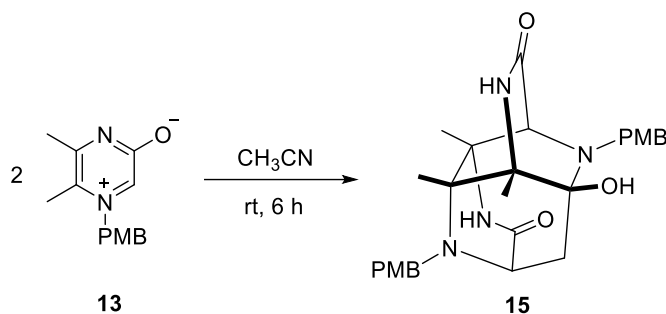
Scheme 5. Dimerization of 3-oxopyrazinium 13 .
