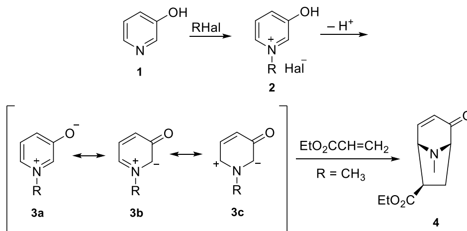
Scheme 1. Main resonance contributors to 3-oxidopyridiniums and reaction of 1-methyl-3-oxidopyridinium 3 (R=Me) with ethyl acrylate.
