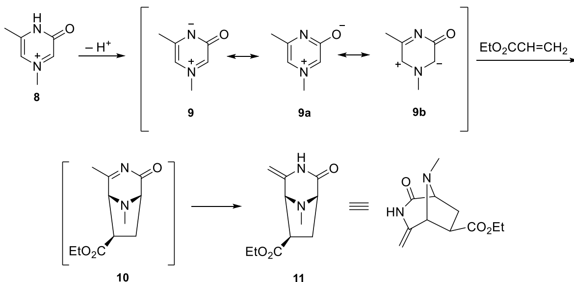
Scheme 3. Synthesis of 3-oxido-1,5-dimethylpyrazinium ( 9 ) and its reaction with ethyl acrylate
